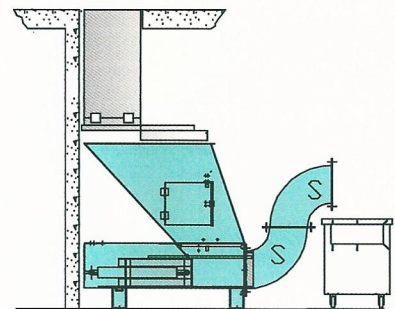
SIDE VIEW "S" & "S" SECTIONS FRONT DISCHARGE
