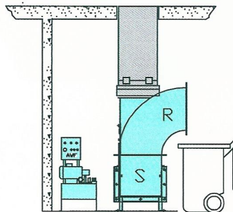
FRONT VIEW "S" & "R" SECTIONS SIDE DISCHARGE
