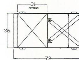
TOP SECTIONAL VIEW
