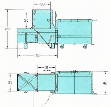
A630-HF LAYOUT WITH 2CY RL CONTAINER
